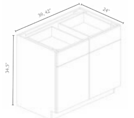
DOUBLE DOOR, DOUBLE DRAWER
