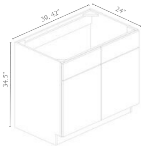
DOUBLE DOOR, DOUBLE DRAWER
